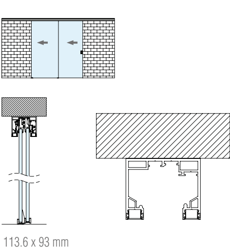
TELESCOPICO A SOFFITTO Telescopic on Ceiling
