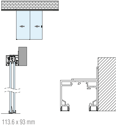
TELESCOPICO A PARETE Telescopic on Wall
